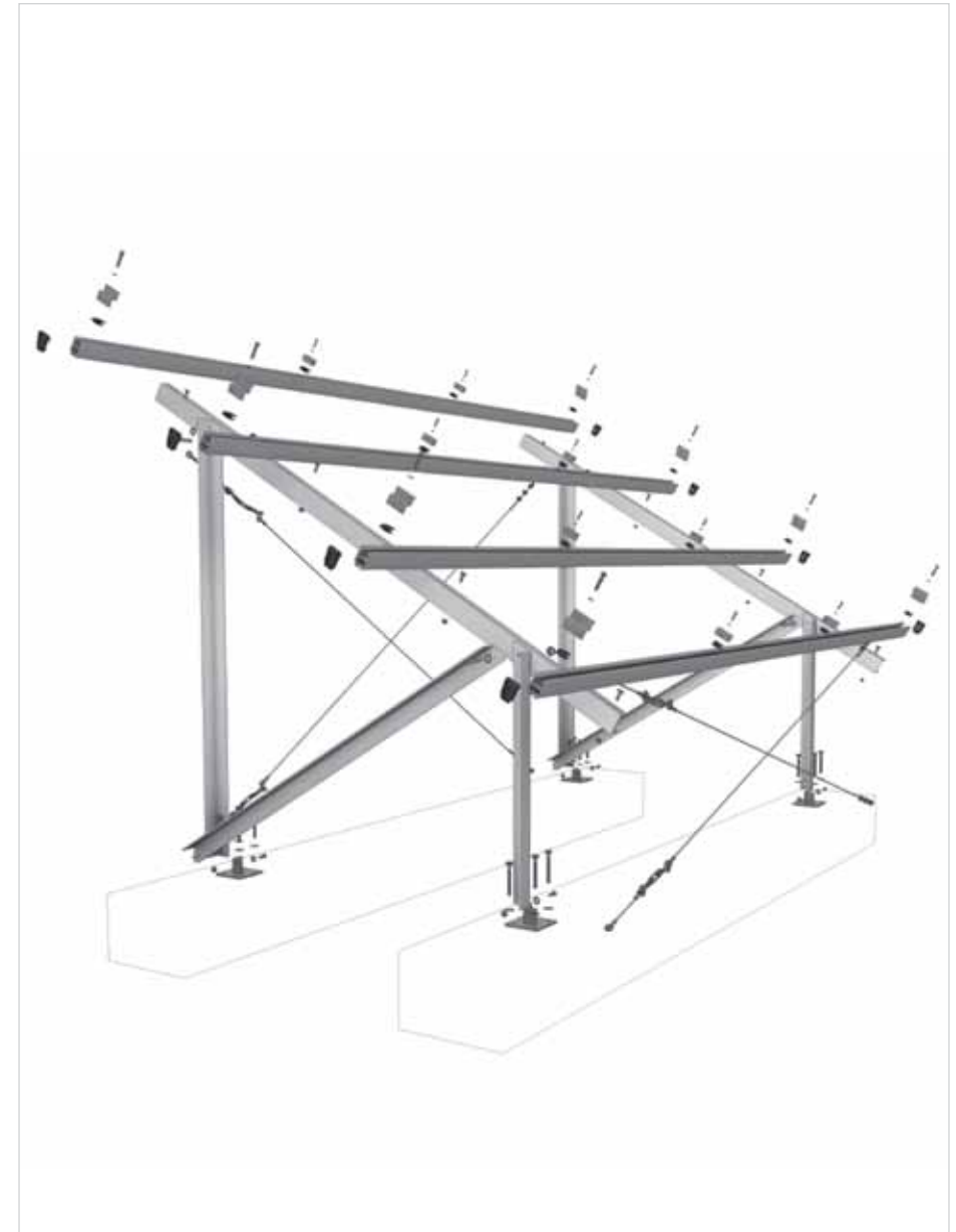
Explosion drawing - N-Rack System Mono
